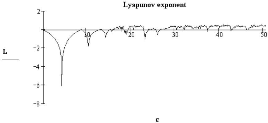
Figure 2. Lyapunov exponent for function, with varying \varepsilon parameter
